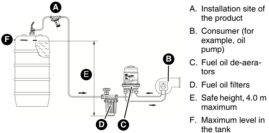
Fig. 7: Safe height = height difference between maximum level in the tank and lowest point of the supply line
