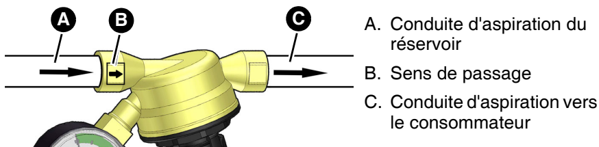
Figure 4: Montage
